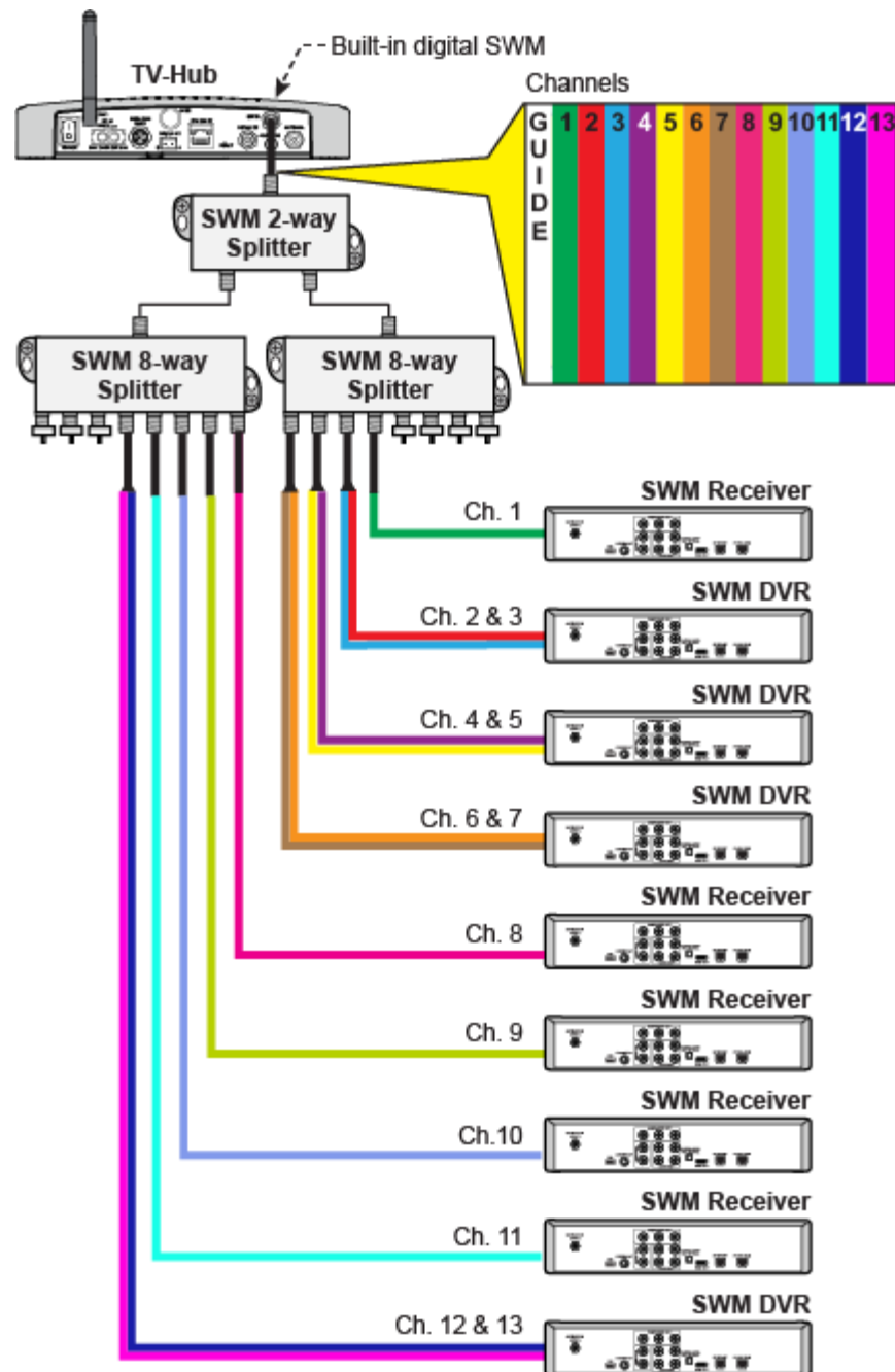
Figure 7-6 DIRECTV SWM Technology
