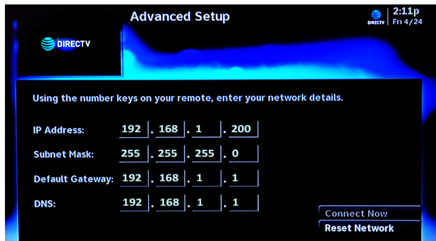
Figure 5-5 IP Address on a DIRECTV Receiver WITH an Onboard Network (Example)
