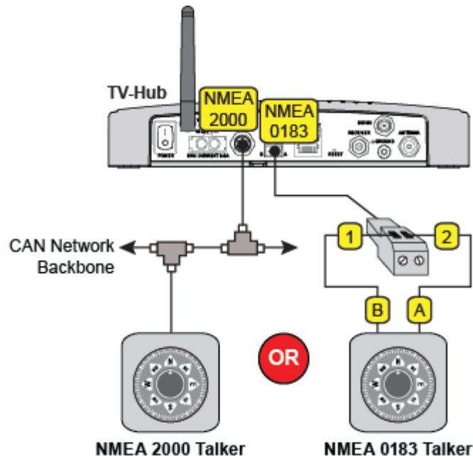
Figure 4-1 TV-Hub NMEA Connections
