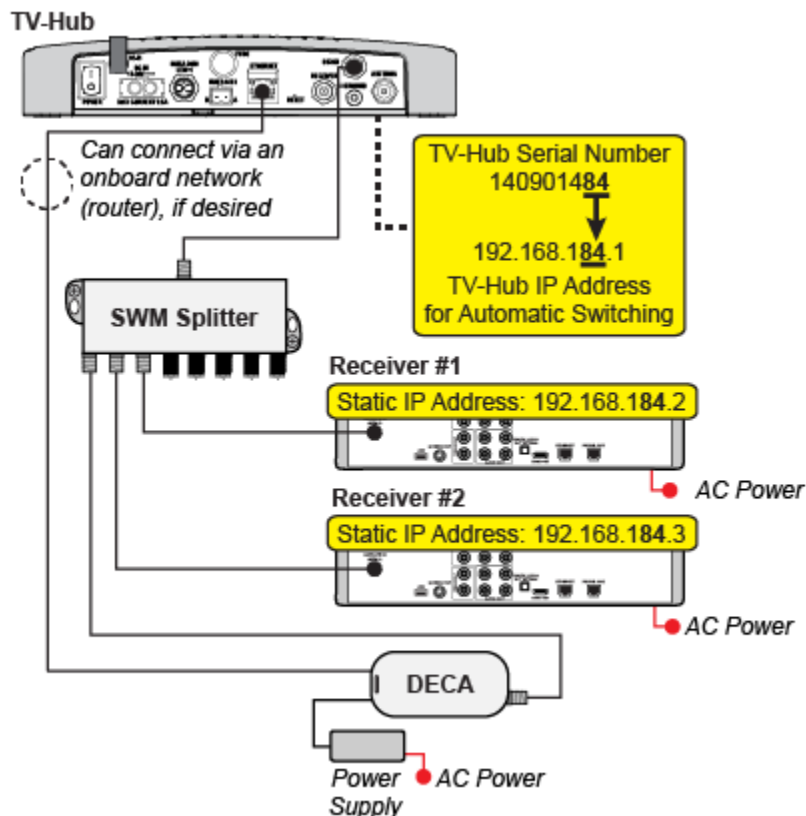
Figure 5-2 IP Addressing for Automatic Switching (Example)
