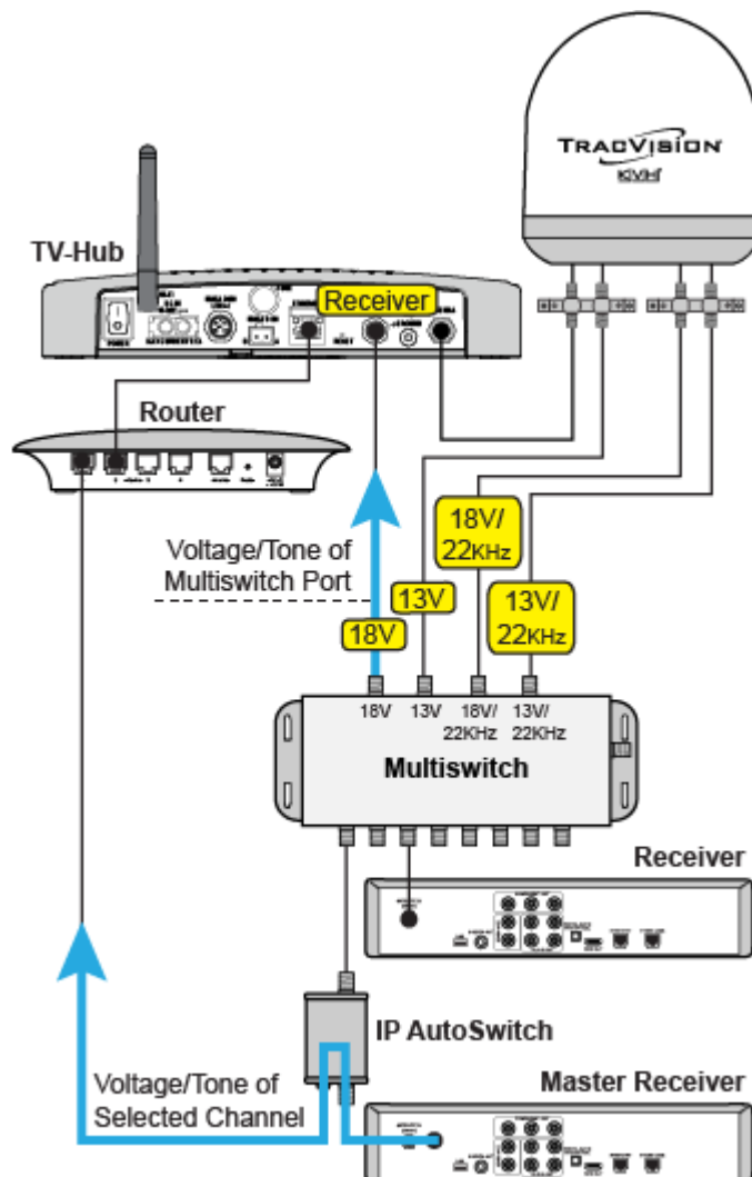
Figure 4-2 Example of Conflicting Band/Polarization Requests
