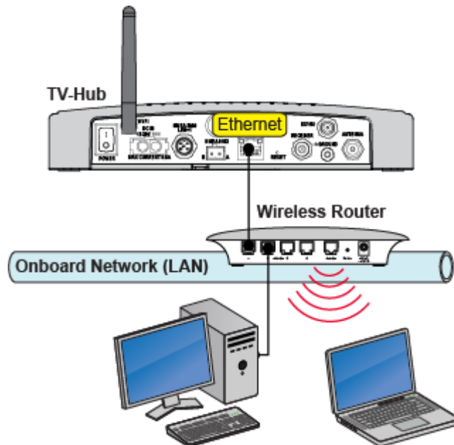
Figure 3-1 TV-Hub Wired Network Connection
