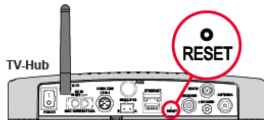
Figure 3-6 Reset Button
