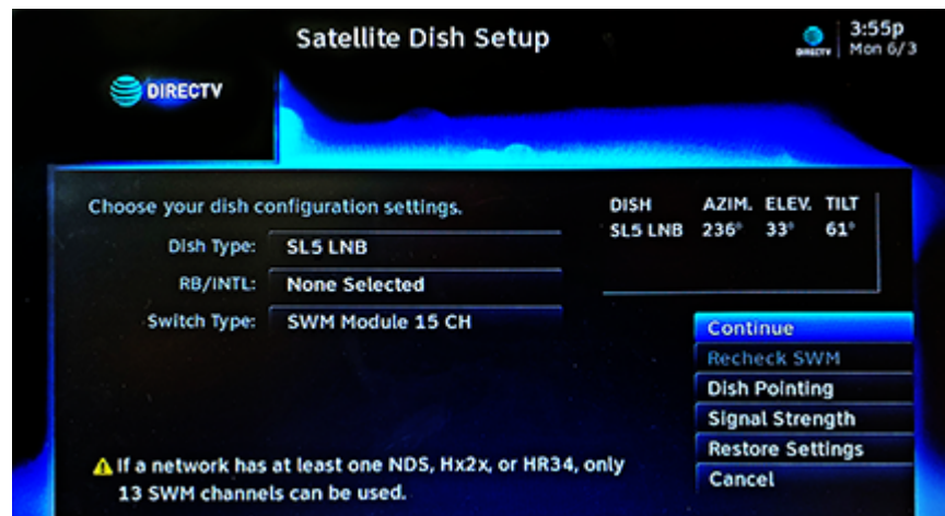
Figure 5-7 Dish Setup Menu on DIRECTV Receiver (Example)
