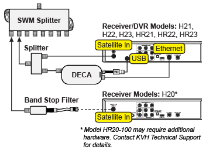
Figure 7-4 Additional Equipment for Older Receivers
