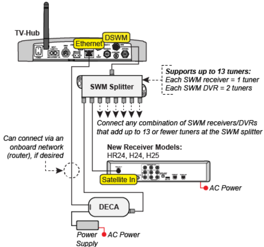
Figure 7-3 DIRECTV Coax Configuration
