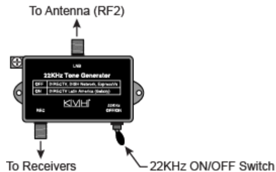
Figure 7-11 22KHz Tone Generator
