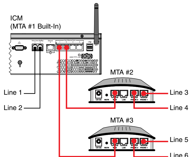
Figure 6-4 Multiple MTA Connections
