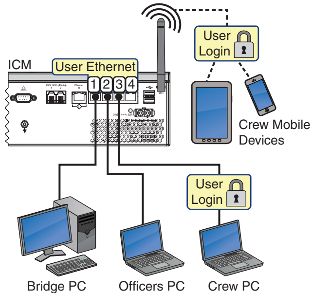
Figure 7-13 Crew-2 Configuration Wiring Example
