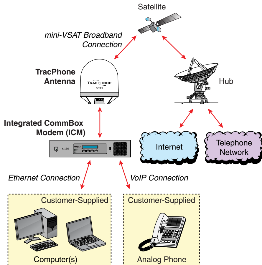
Figure 1-2 TracPhone V11-IP mini-VSAT Broadband Network Diagram
