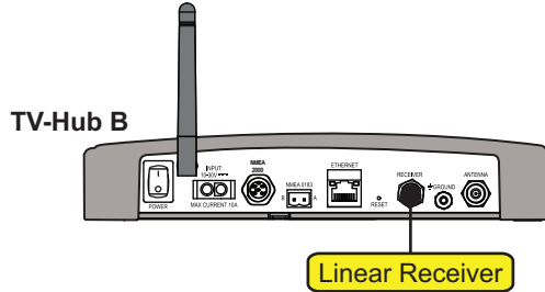
Figure 23: TV-Hub B Receiver Connections
