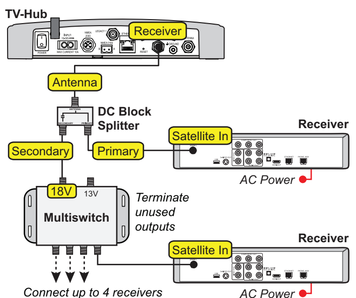
Figure 33: Wiring 3+ DISH/Bell Receivers
