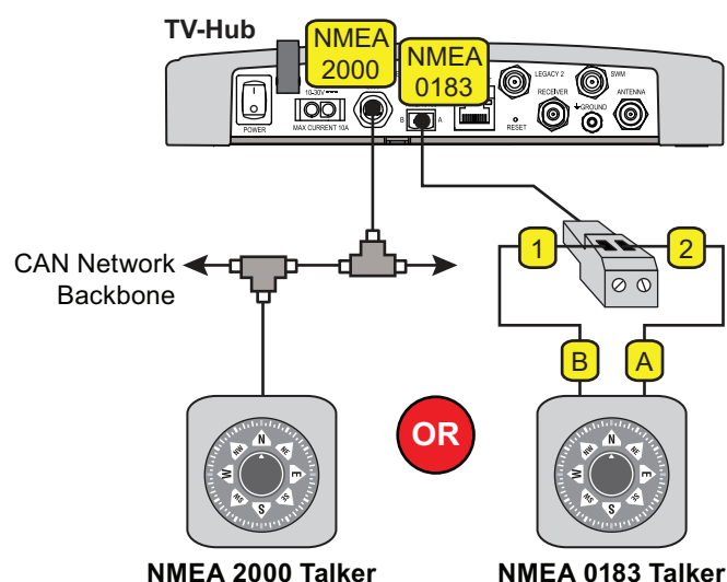
Figure 34: TV-Hub NMEA Connections
