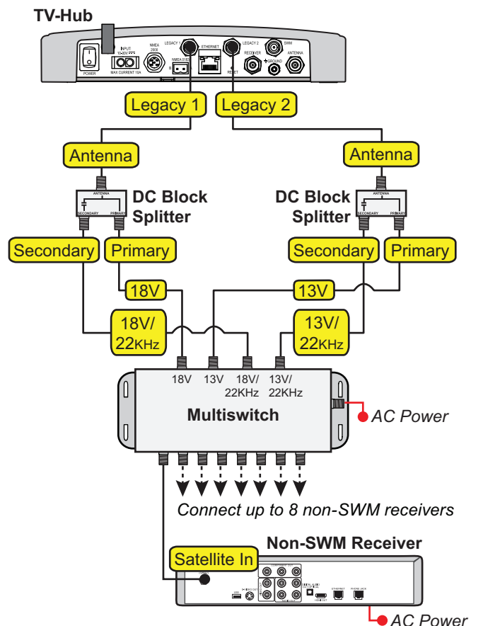
Figure 30: Wiring 3+ DIRECTV Non-SWM Receivers
