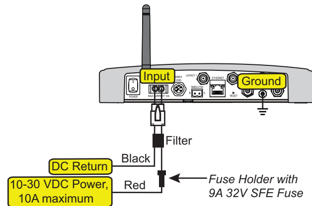
Figure 38: TracVision System Power
