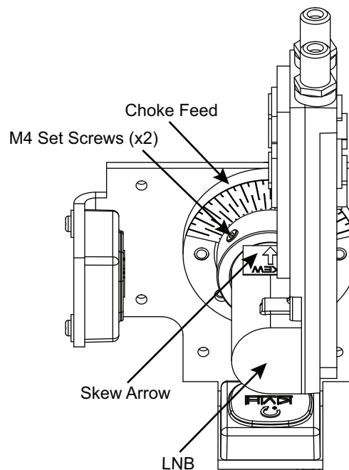
Figure 52: LNB Set Screws and Skew Angle Adjustment
