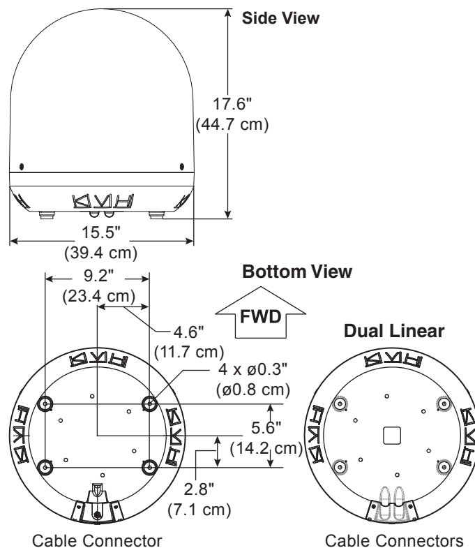
Figure 5: Antenna Dimensions
