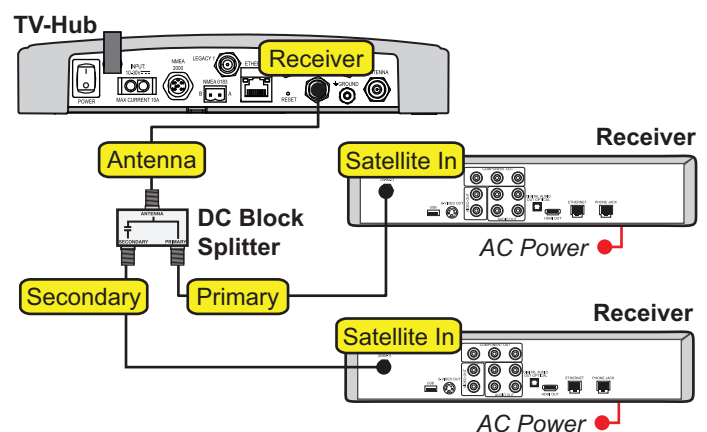
Figure 32: Wiring 2 DISH/Bell Receivers
