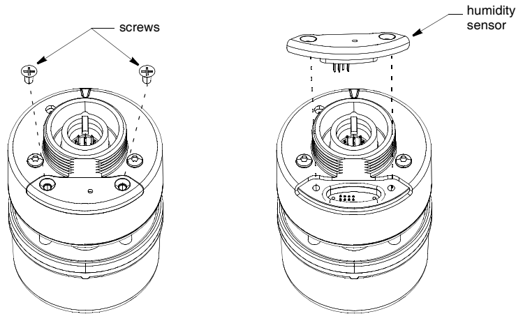
Figure 11. Replacing the humidity sensor
