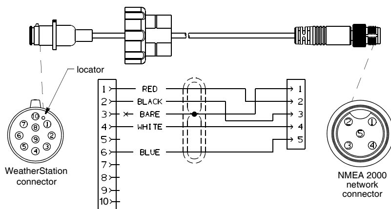
Figure 8. NMEA 2000® WeatherStation Cable [6m (20') shown]
