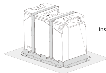
*Battery Mounting Strap
