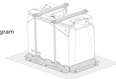
*Battery Mounting Bracket
