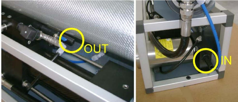
CONCENTRATE OUTLET (OUT) AND SEAWATER INLET (IN) FIG. 3-8
