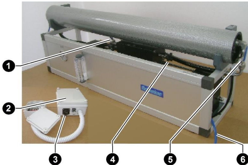
WATERMAKER GROUP (LATERAL VIEW) FIG. 3-7
