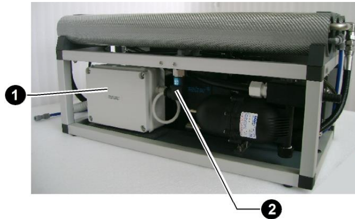
WATERMAKER GROUP (BACK VIEW) FIG. 3-8
