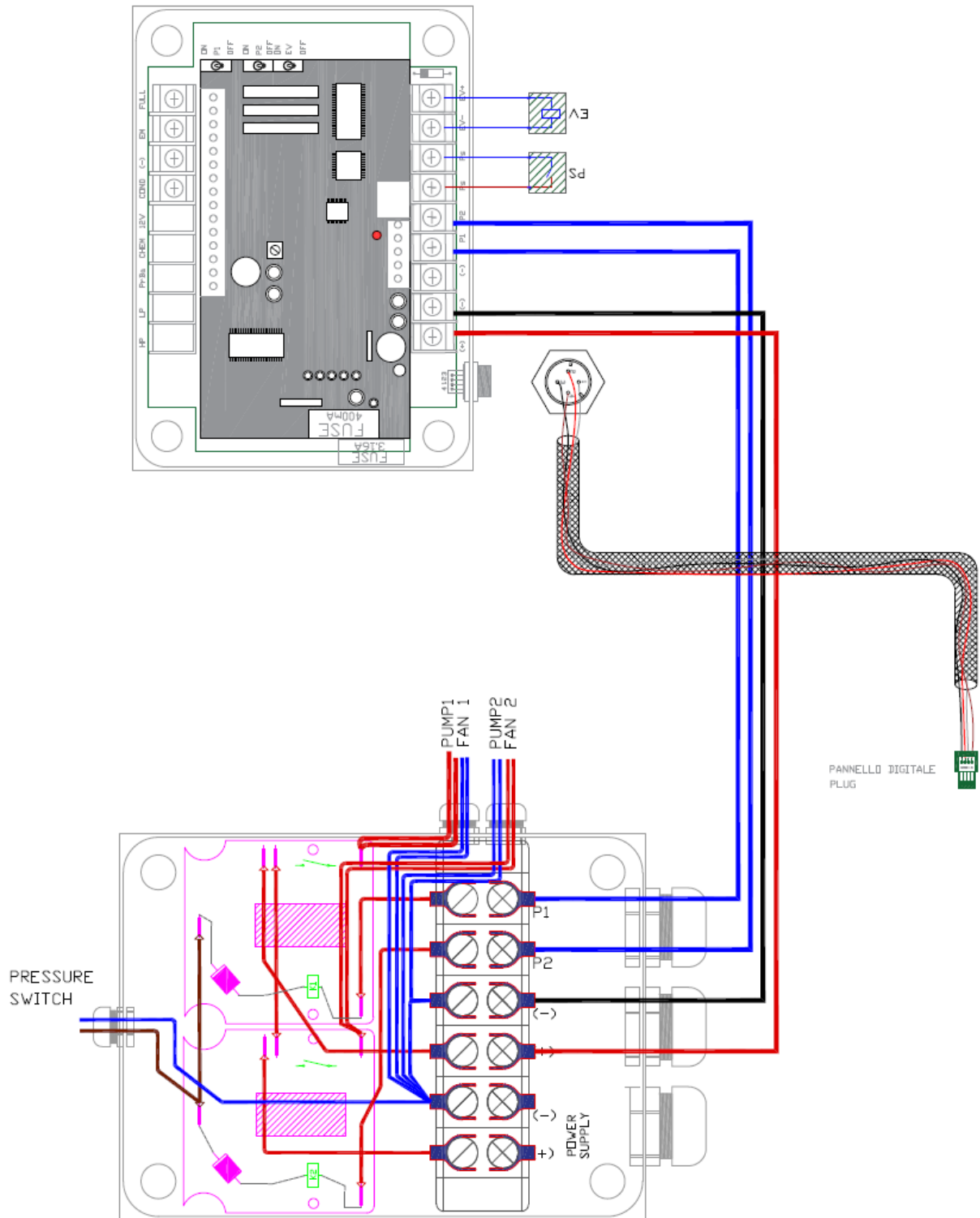
ELECTRIC MAIN BOX SCHEME MODULAR 60 12/24V DC FIG. 4-5
