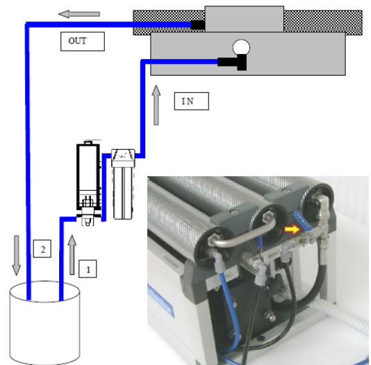
HYDRAULIC SCHEME FOR WINTERIZING PROCEDURE FIG. 6-2
