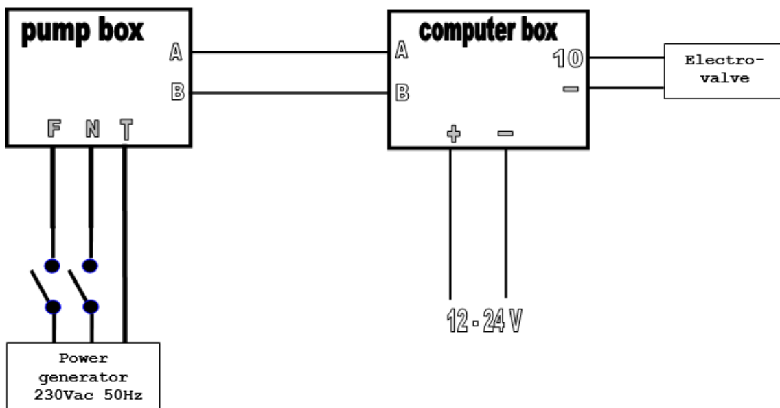
WIRING LOGIC SCHEME 230 VAC FIG. 4-4
