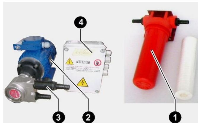
PUMP GROUP AND FILTER 230 V AC FIG. 3-5
