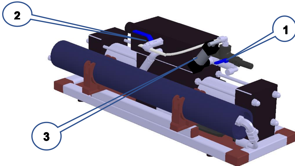
WATERMAKER GROUP (BACK VIEW) FIG. 3-7
