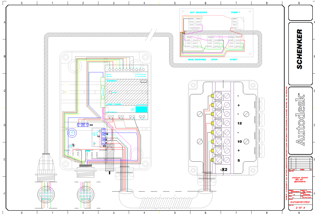
ELECTRIC MAIN BOX SCHEME WITH REMOTE PANEL SMART 30 12/24V DC FIG. 4-5
