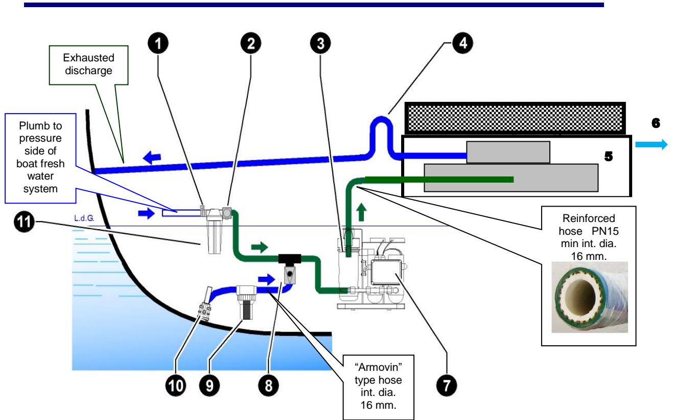
HYDRAULIC CONNECTION AND PIPES
