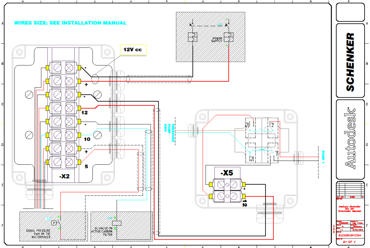
ELECTRIC MAIN BOX SCHEME SMART 30 12/24V DC FIG. 4-4
