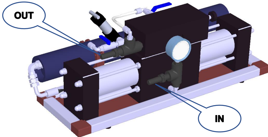
CONCENTRATE OUTLET (OUT) AND SEAWATER INLET (IN) FIG. 3-8
