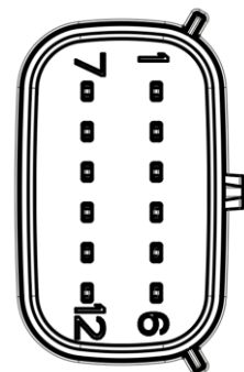
Molex MX150 12-poles Code A connector, display pin view
