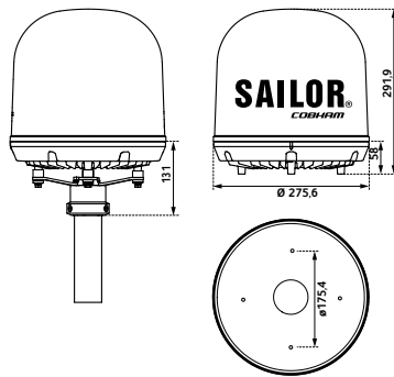
SAILOR 150 FleetBroadband Above Deck Unit (3,9 kg)
